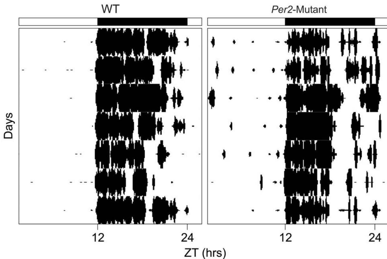
Figure S3 Per2-mutant mice exhibit daily rhythms in wheel-running activity Mice were placed in cages with access to a running wheel and wheel-running activity was recorded. Examples of wheel-running activity from a WT mouse (left-hand panel) and a Per2-mutant mouse (right-hand panel) are shown. Bars at the top of the panels indicate the LD cycle. All of the mice evaluated exhibited daily rhythms in activity.
